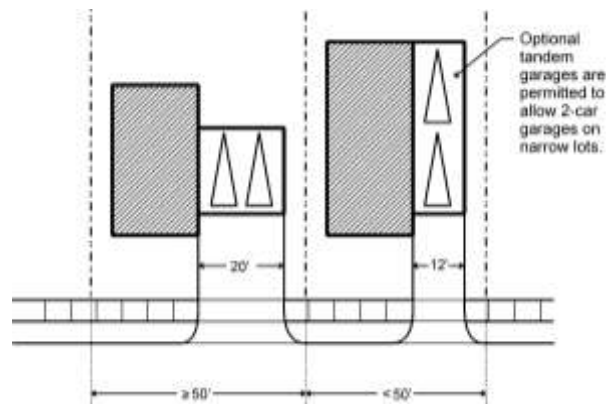
Figure 3. Driveway standards.
