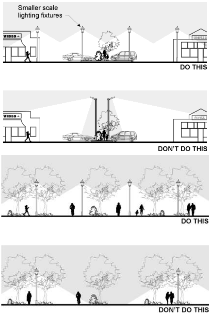
Figure 35. Lighting guidelines.
