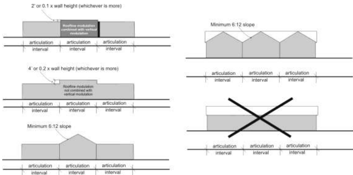
Figure 44. Roofline modulation standards.
