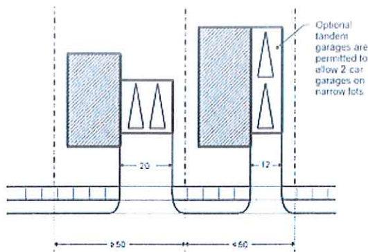
Figure 3. Driveway standards.
